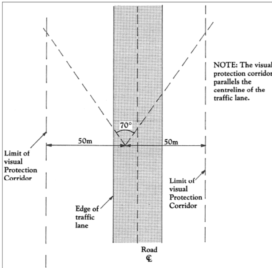
Diagram 1 – Visual Protection Corridor Diagram not to scale
